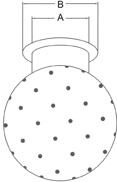
Tri-Clamp管夾固定式 STATIC with Tri-Clamp Connection
